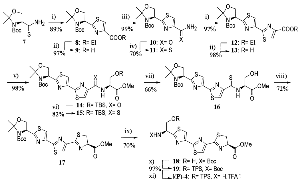
Scheme 1. Reagents and conditions: i) a) \text{KHCO}_3 , ethyl 3-bromopyruvate, DME, 0 °C, 30 min, rt, 2 h, b) TFAA, pyridine, DME, 0 °C, 1 h, ii) 1 M LiOH, \text{H}_2\text{O} -dioxane (1:1 v/v), 0 °C, 30 min, rt, 3 h, iii) a) \text{ClCOOEt} , \text{Et}_3\text{N} , THF, 0 °C, 30 min, b) 28% aq \text{NH}_3 , THF, 0 °C, 5 min, iv) Lawesson's reagent, DME, rt, 10 h, v) H-Ser(TBS)-OMe, DPPA, \text{Et}_3\text{N} , DMF, 0 °C, 30 min, rt, 9 h, vi) Lawesson's reagent, 50 °C 16 h, vii) TBAF, THF, 0 °C 1 h, viii) \text{Ph}_3\text{P} , DEAD, THF, 0 °C, 1 h, ix) TFA- \text{CHCl}_3 (4:96 v/v), rt, 2 h, x) TPSCl, imidazole, \text{CHCl}_3 , 0 °C, rt, 12 h, xi) THF- \text{CHCl}_3 (2:3 v/v), rt, 30 min.
