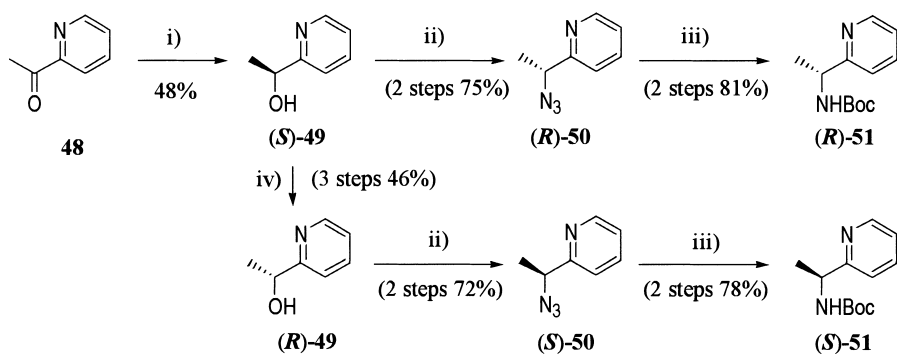
Scheme 4. Reagents and conditions: i) Baker's Yeast, D-Glucose, H 2 O, 48 h, ii) a) MsCl, Et 3 N, CHCl 3 , 0 °C, 30 min, b) NaN 3 , DMF, rt, overnight, iii) a) H 2 , 10% Pd-C, EtOH, rt, 30 min, b) Boc 2 O, Et 3 N, CHCl 3 , 0 °C, 30 min, rt, 3 h, iv) a) MsCl, Et 3 N, 0 °C, 30 min, b) NaOAc, 15-crown-5-ether, DMF, rt, 24 h, c) K 2 CO 3 , MeOH, H 2 O, 0 °C, 30 min, rt, 3 h.
