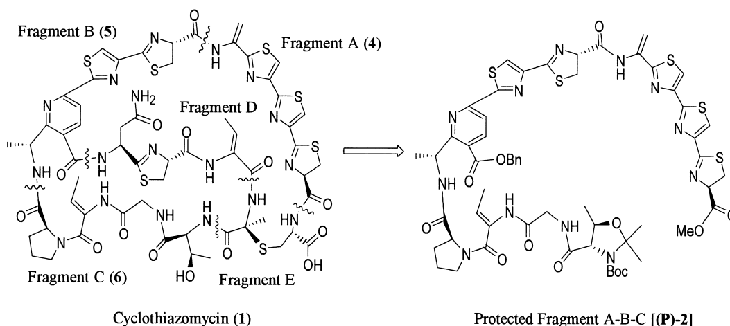
Fig. 1. Retrosynthesis of 1 .
